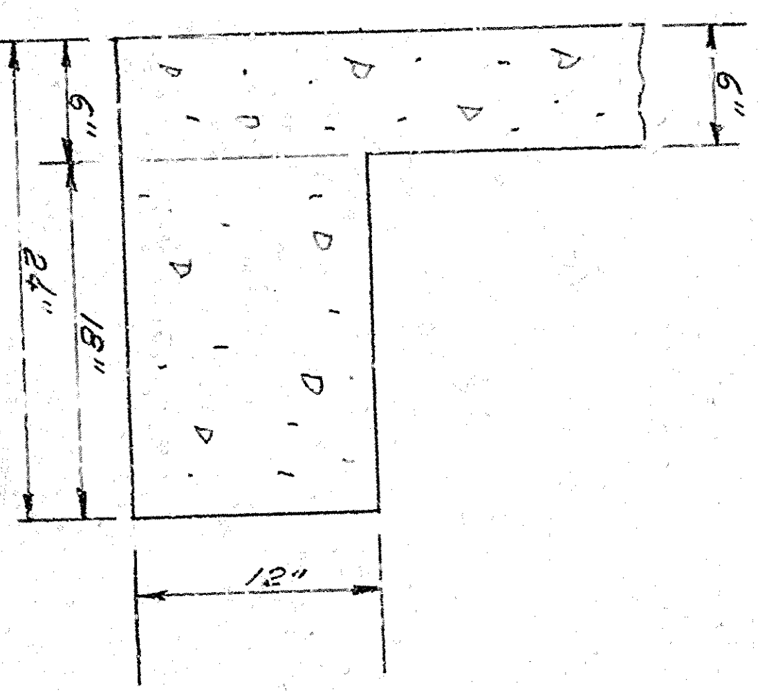
SPREAD FOOTING
