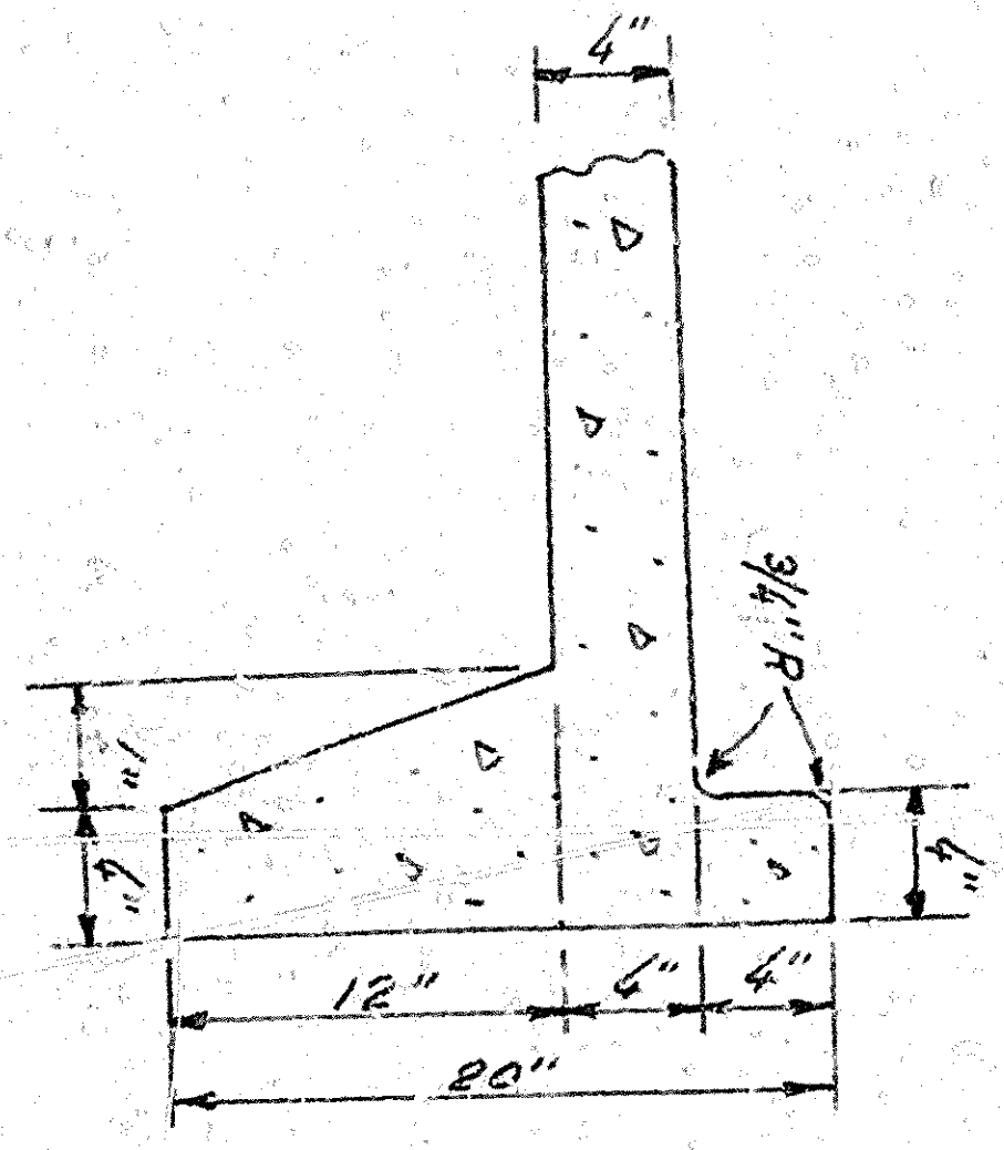
CURB DETAIL
